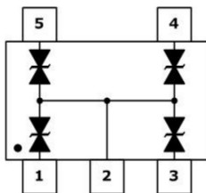
Circuit and Pin Schematic
